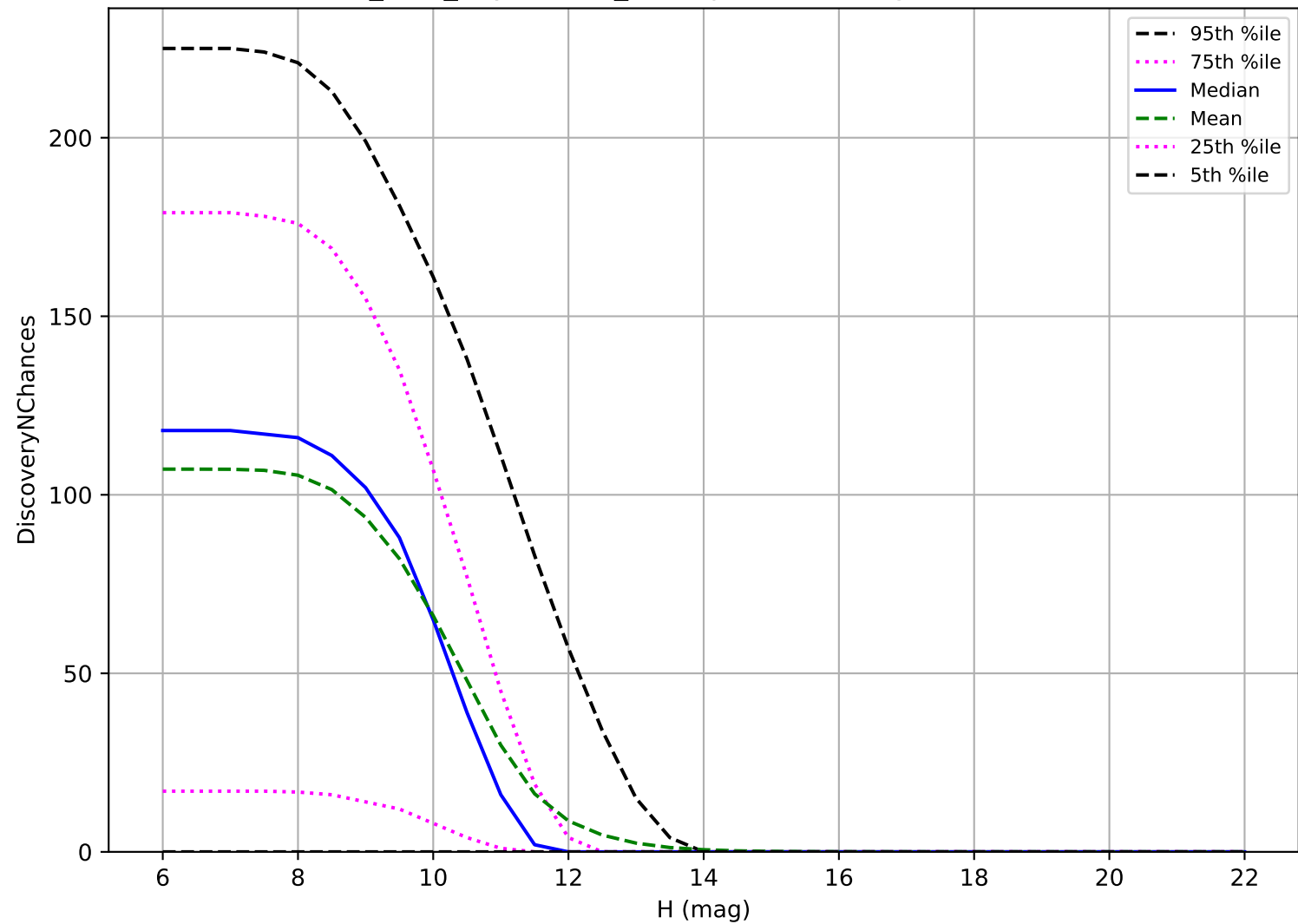
baseline_v3.3_10yrs: OCC_r20 3 pairs in 15 nights detection loss
