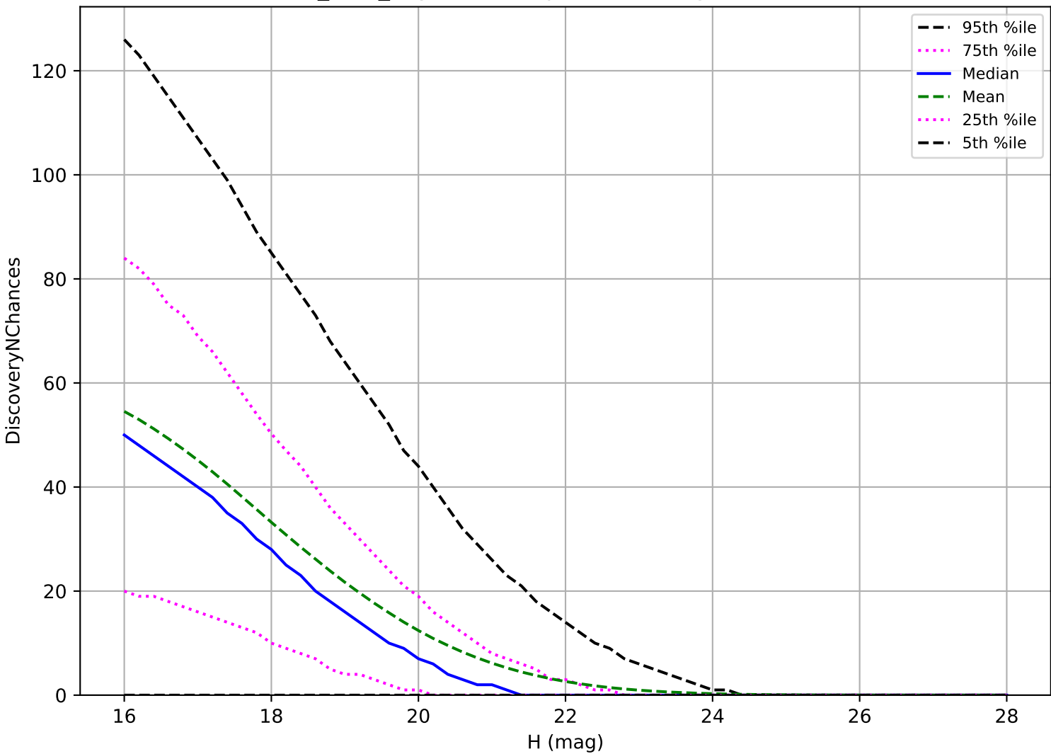
baseline_v3.3_10yrs: NEO 3 pairs in 15 nights detection loss
