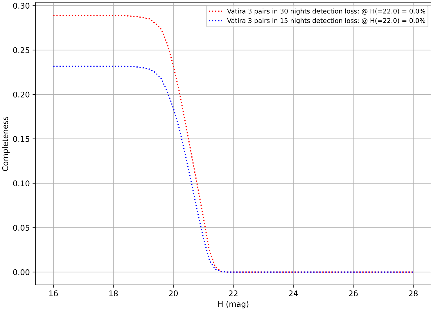
baseline_v3.3_10yrs: DifferentialCompleteness
