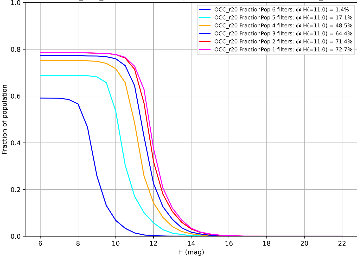
baseline_v3.3_10yrs: Fraction of population with colors in X filters OCC_r20
