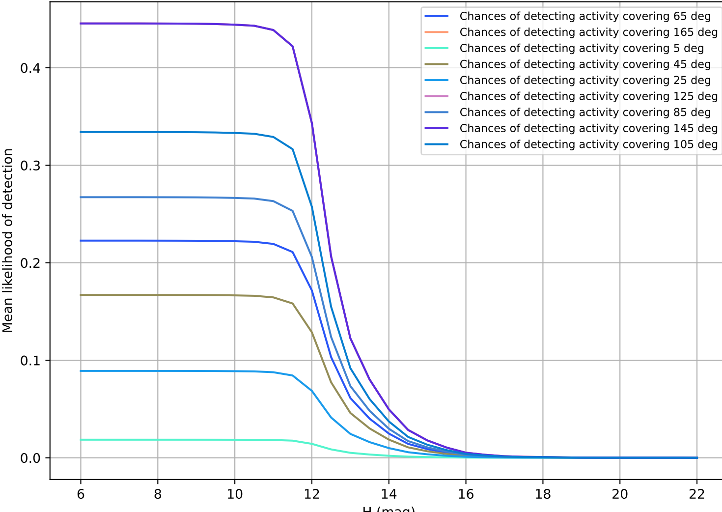
baseline v3.3 10yrs OCC r20
