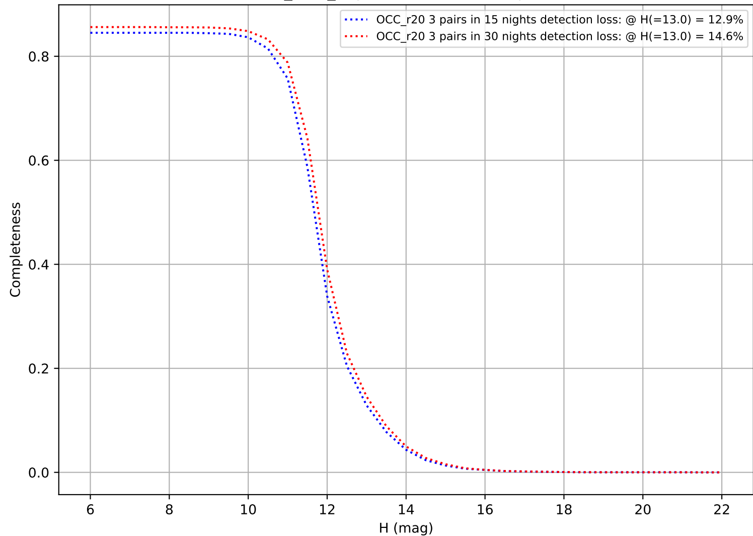
baseline_v3.3_10yrs: DifferentialCompleteness
