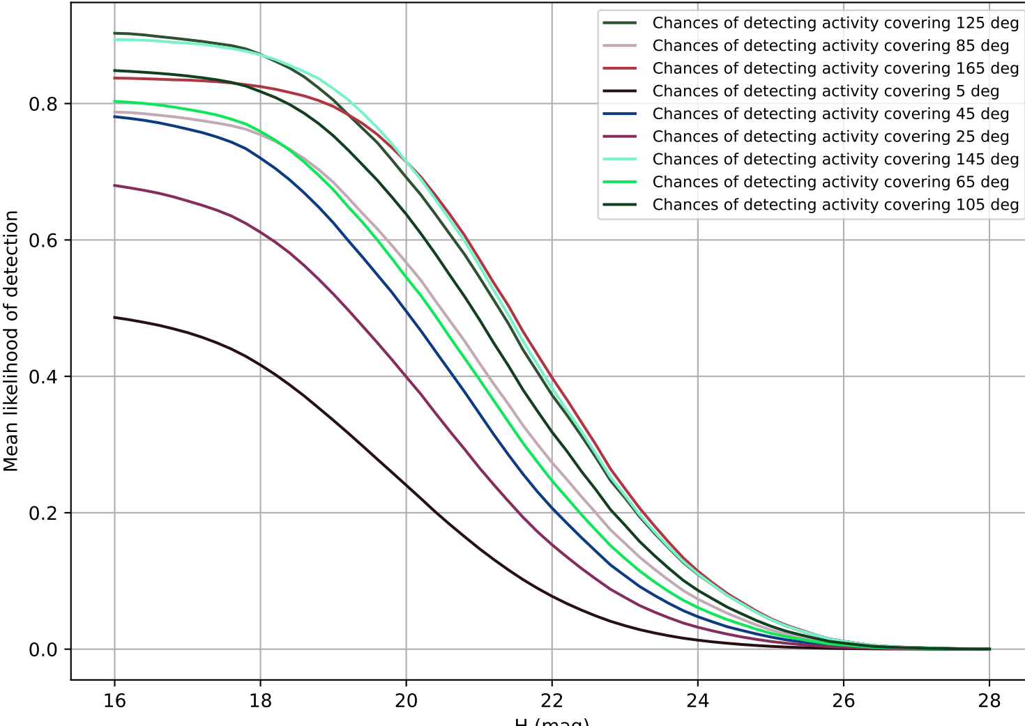
baseline v3.3 10yrs NEO
