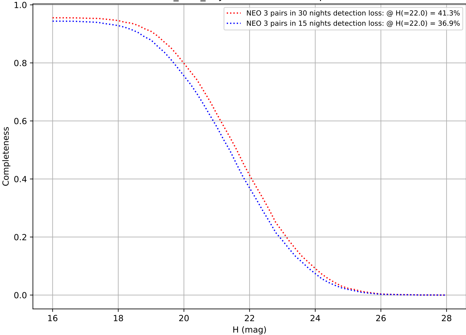
baseline_v3.3_10yrs: DifferentialCompleteness
