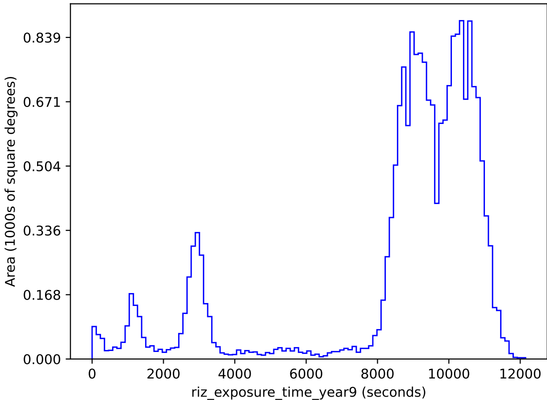
baseline_v3.3_10yrs gri band non-DD: riz_exposure_time_year9
