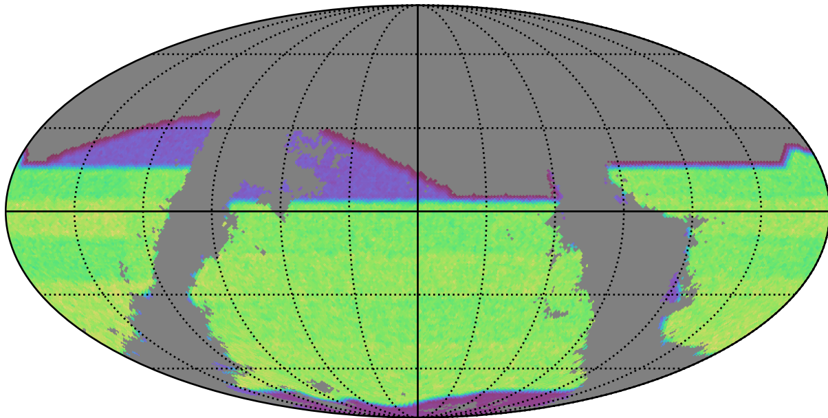
baseline_v3.3_10yrs gri band non-DD: riz_exposure_time_year8
