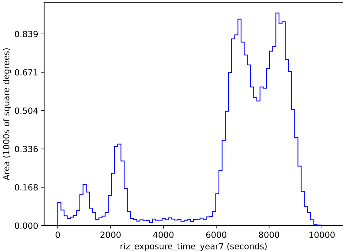
baseline_v3.3_10yrs gri band non-DD: riz_exposure_time_year7
