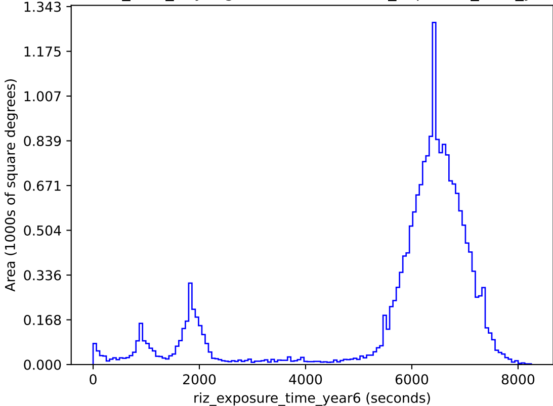
baseline_v3.3_10yrs gri band non-DD: riz_exposure_time_year6
