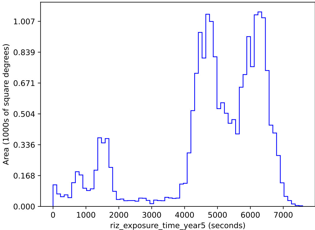
baseline_v3.3_10yrs gri band non-DD: riz_exposure_time_year5
