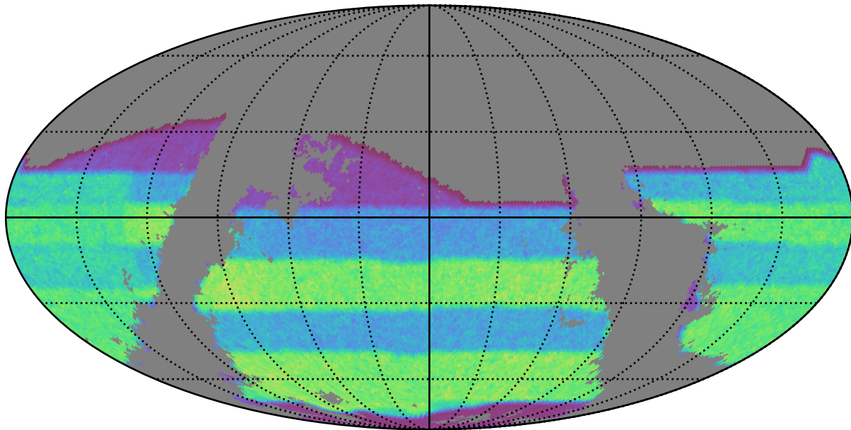
baseline_v3.3_10yrs gri band non-DD: riz_exposure_time_year3
