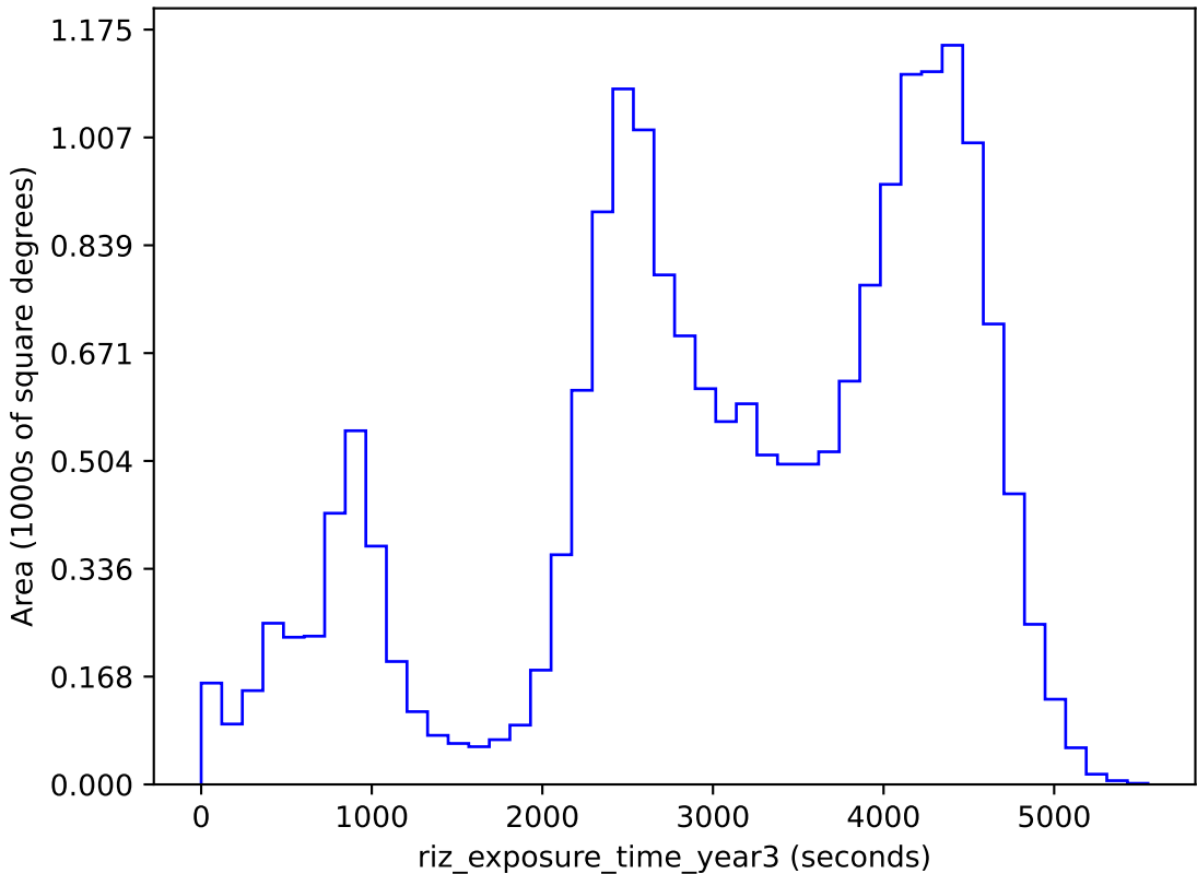
baseline_v3.3_10yrs gri band non-DD: riz_exposure_time_year3
