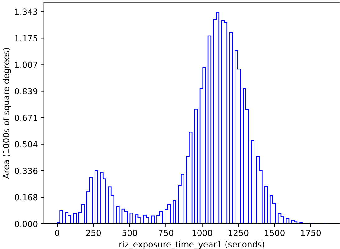
baseline_v3.3_10yrs gri band non-DD: riz_exposure_time_year1
