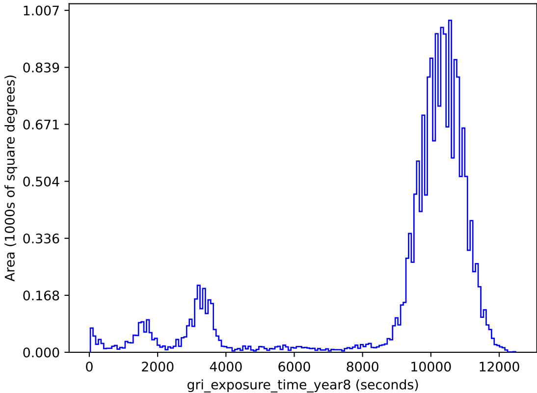
baseline_v3.3_10yrs gri band non-DD: gri_exposure_time_year8
