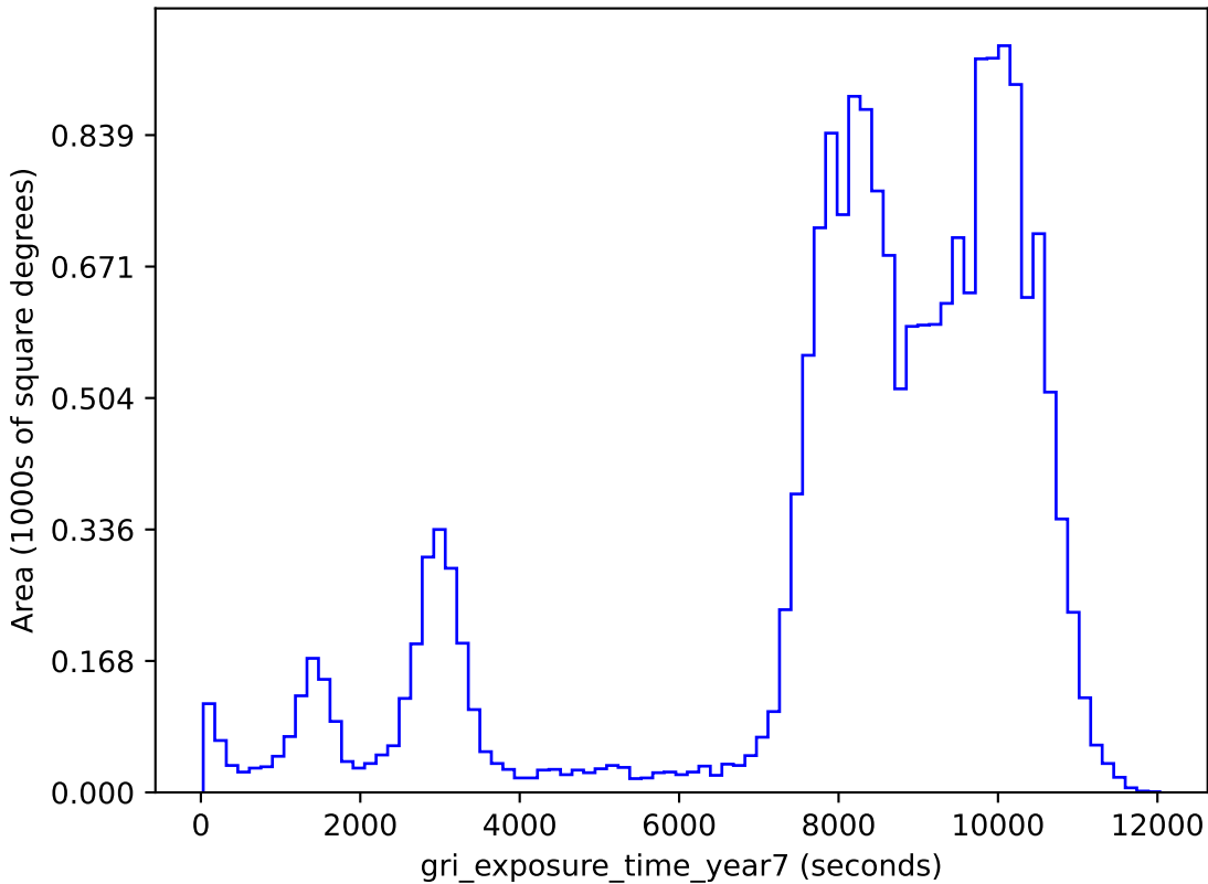
baseline_v3.3_10yrs gri band non-DD: gri_exposure_time_year7
