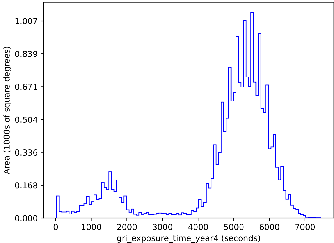
baseline_v3.3_10yrs gri band non-DD: gri_exposure_time_year4
