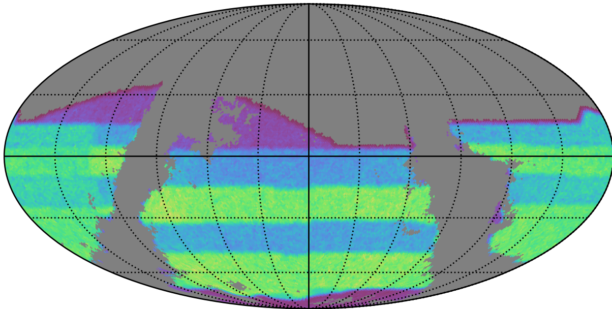
baseline_v3.3_10yrs gri band non-DD: gri_exposure_time_year3
