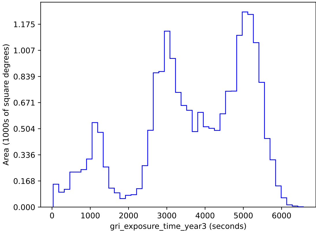
baseline_v3.3_10yrs gri band non-DD: gri_exposure_time_year3
