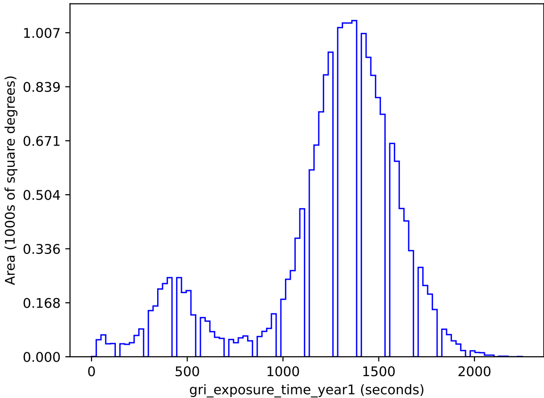
baseline_v3.3_10yrs gri band non-DD: gri_exposure_time_year1
