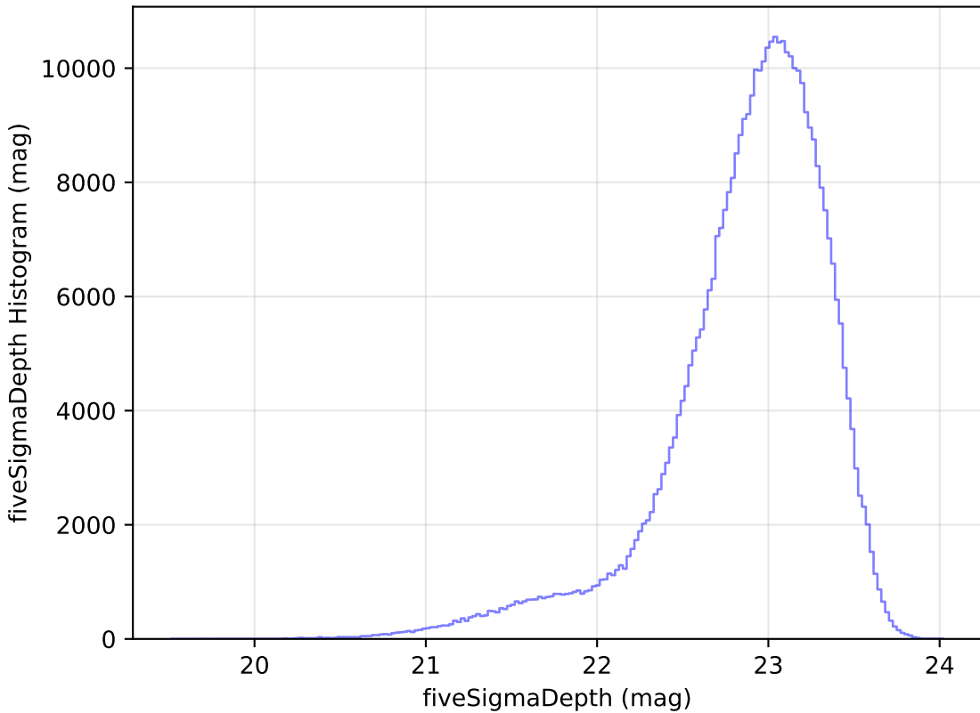
baseline_v3.3_10yrs z: fiveSigmaDepth Histogram
