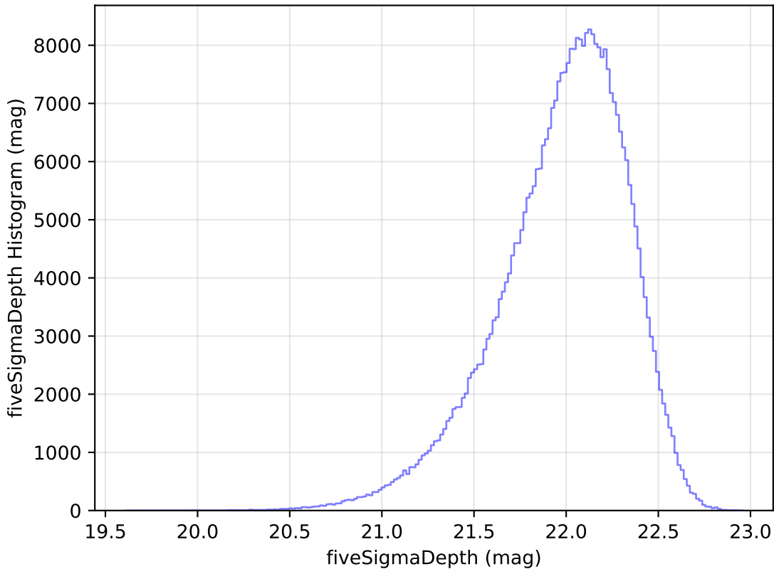
baseline_v3.3_10yrs y: fiveSigmaDepth Histogram
