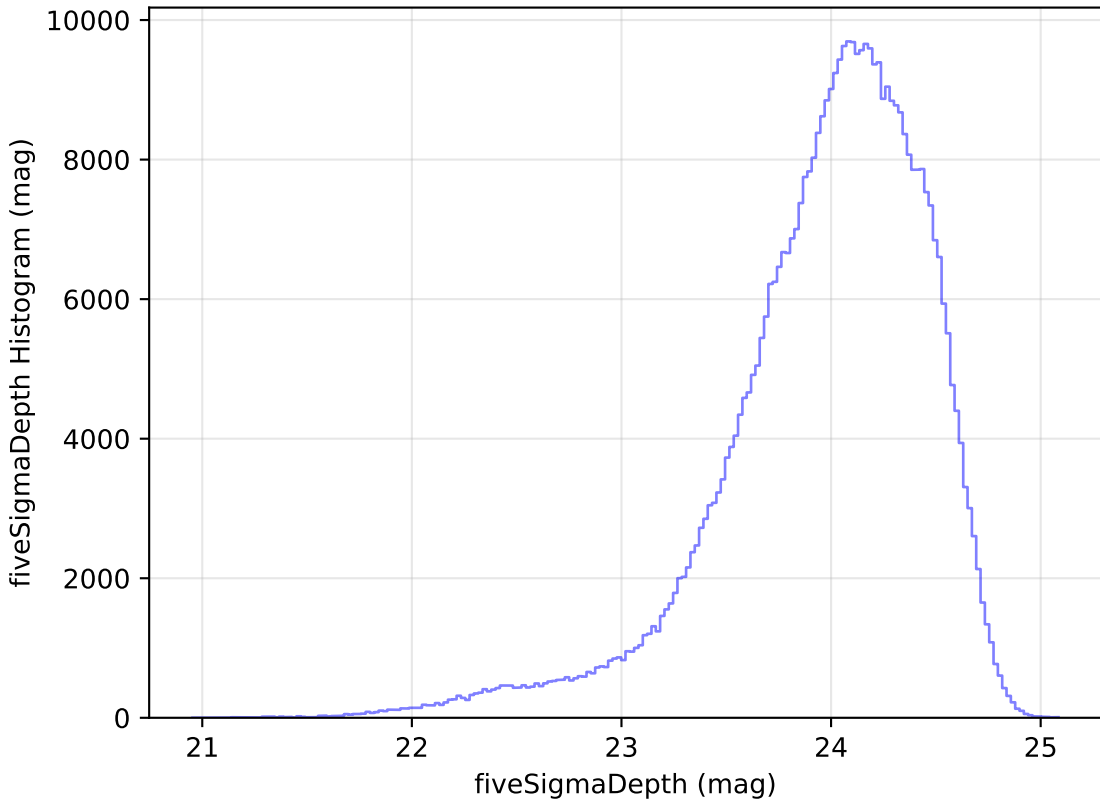
baseline_v3.3_10yrs r: fiveSigmaDepth Histogram
