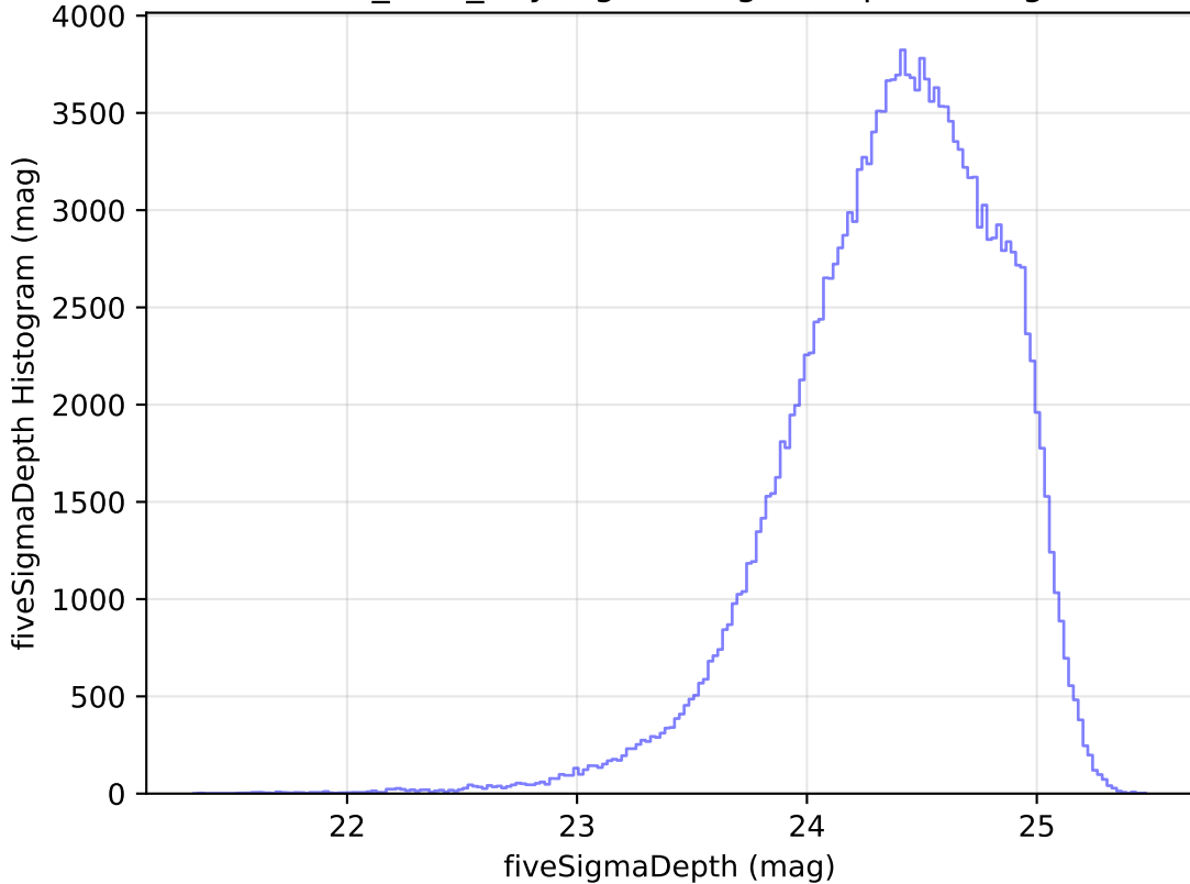
baseline_v3.3_10yrs g: fiveSigmaDepth Histogram
