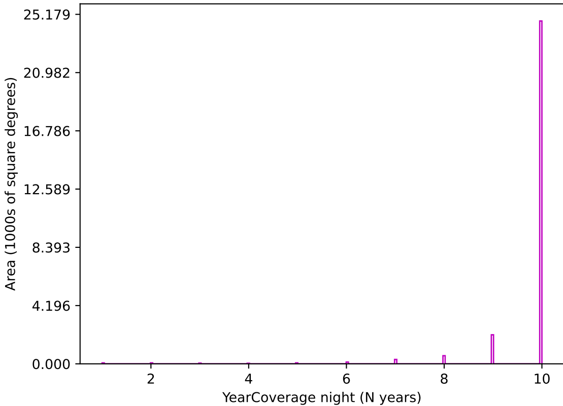
baseline_v3.3_10yrs z band: YearCoverage night
