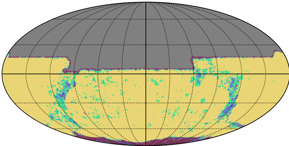
baseline_v3.3_10yrs y band: YearCoverage night
