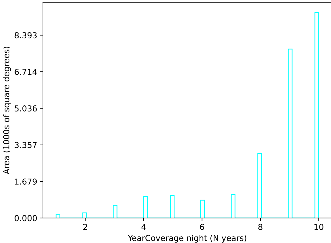
baseline_v3.3_10yrs u band: YearCoverage night
