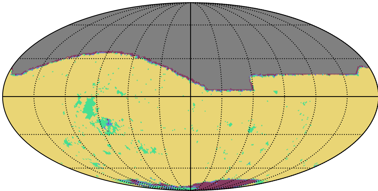
baseline_v3.3_10yrs r band: YearCoverage night
