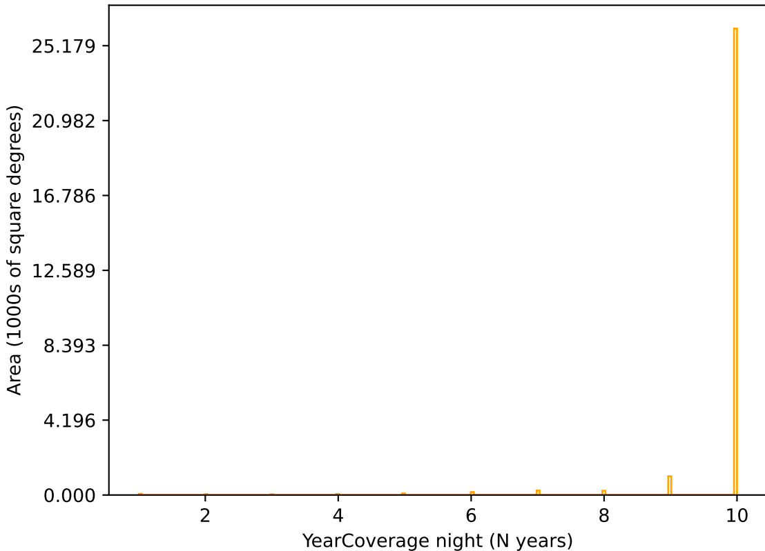
baseline_v3.3_10yrs r band: YearCoverage night
