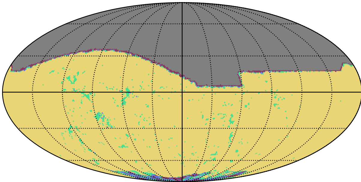
baseline_v3.3_10yrs i band: YearCoverage night
