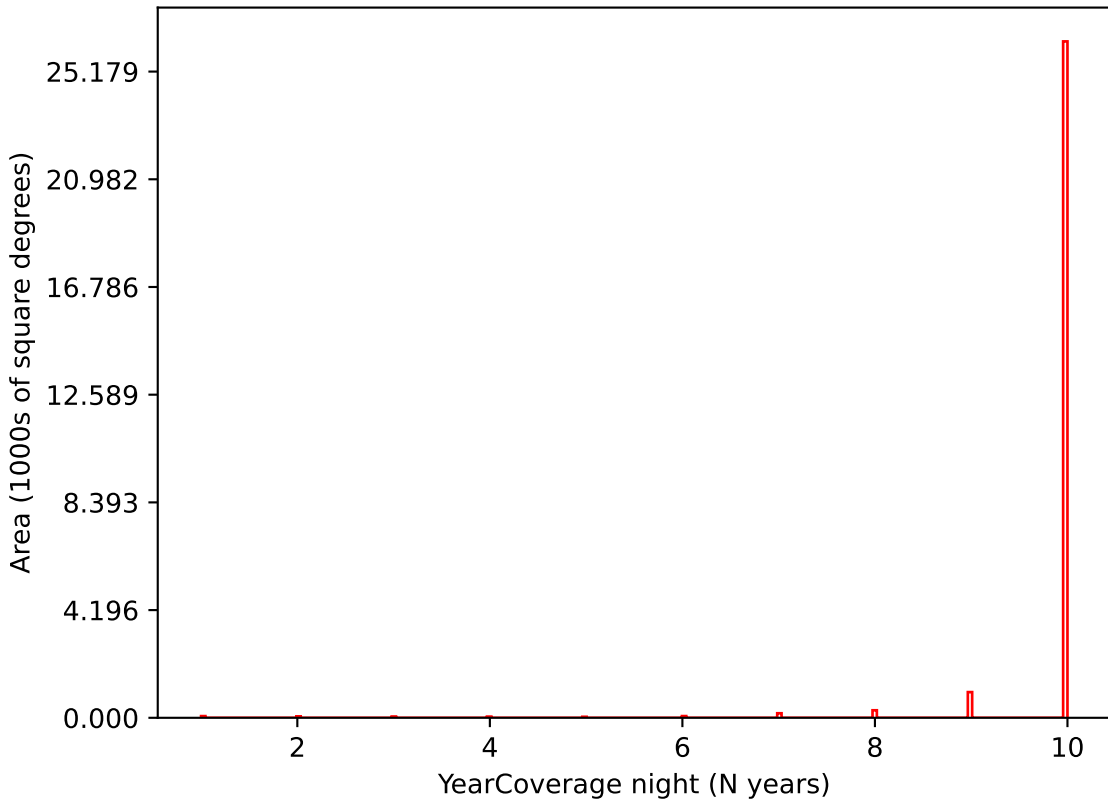
baseline_v3.3_10yrs i band: YearCoverage night
