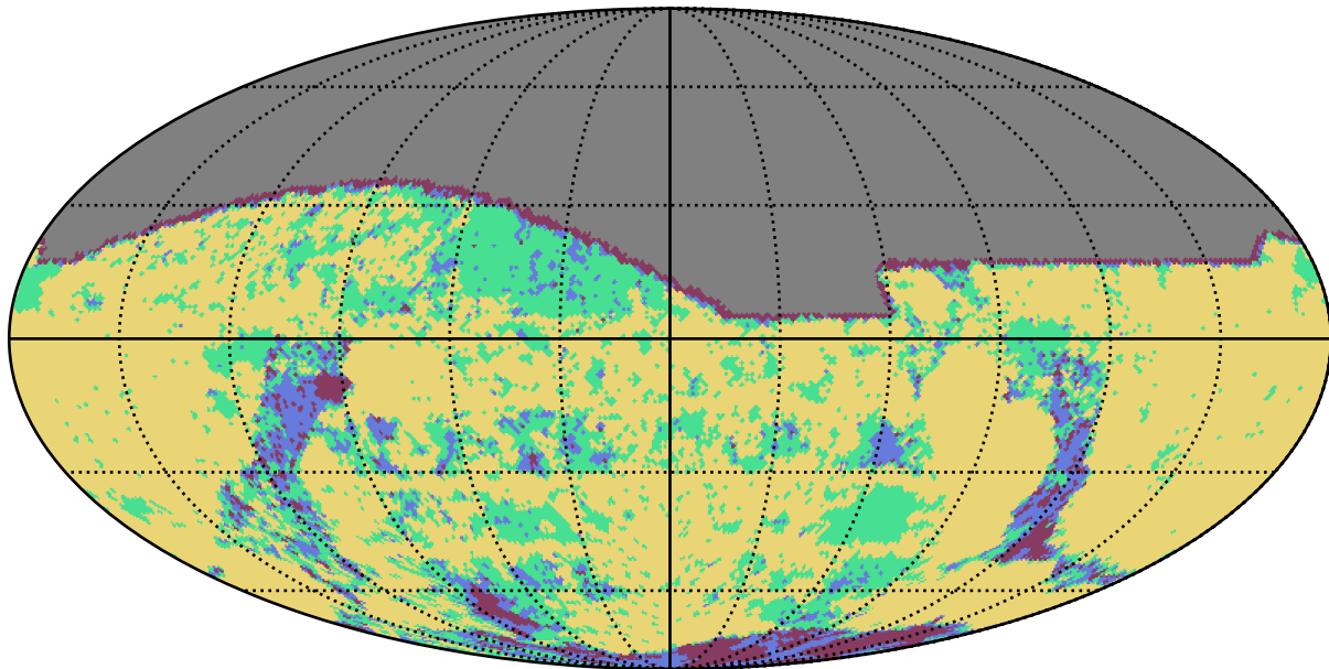
baseline_v3.3_10yrs g band: YearCoverage night
