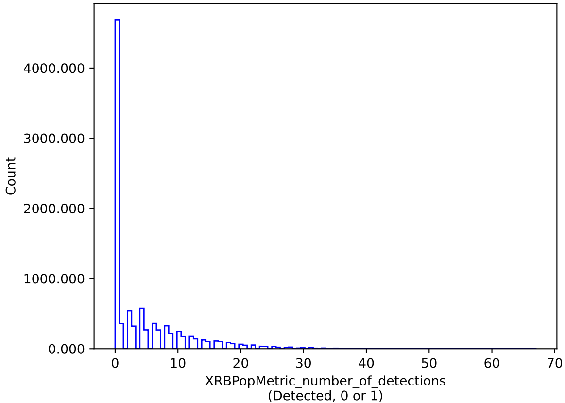
baseline_v3.3_10yrs : XRBPopMetric_number_of_detections
