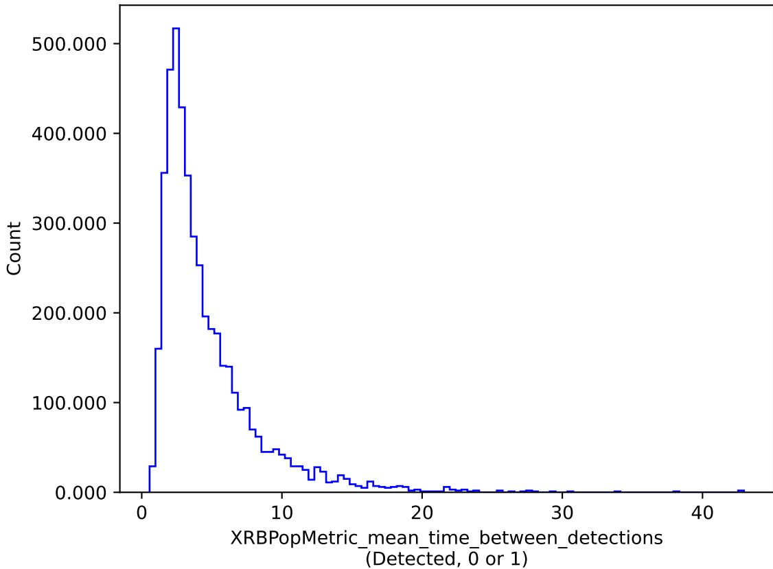
baseline_v3.3_10yrs : XRBPoMetric_mean_time_between_detections
