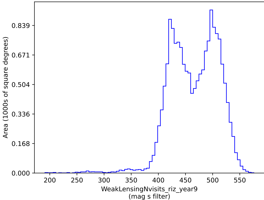
baseline_v3.3_10yrs gri band non-DD: WeakLensingNvisits_riz_year9
