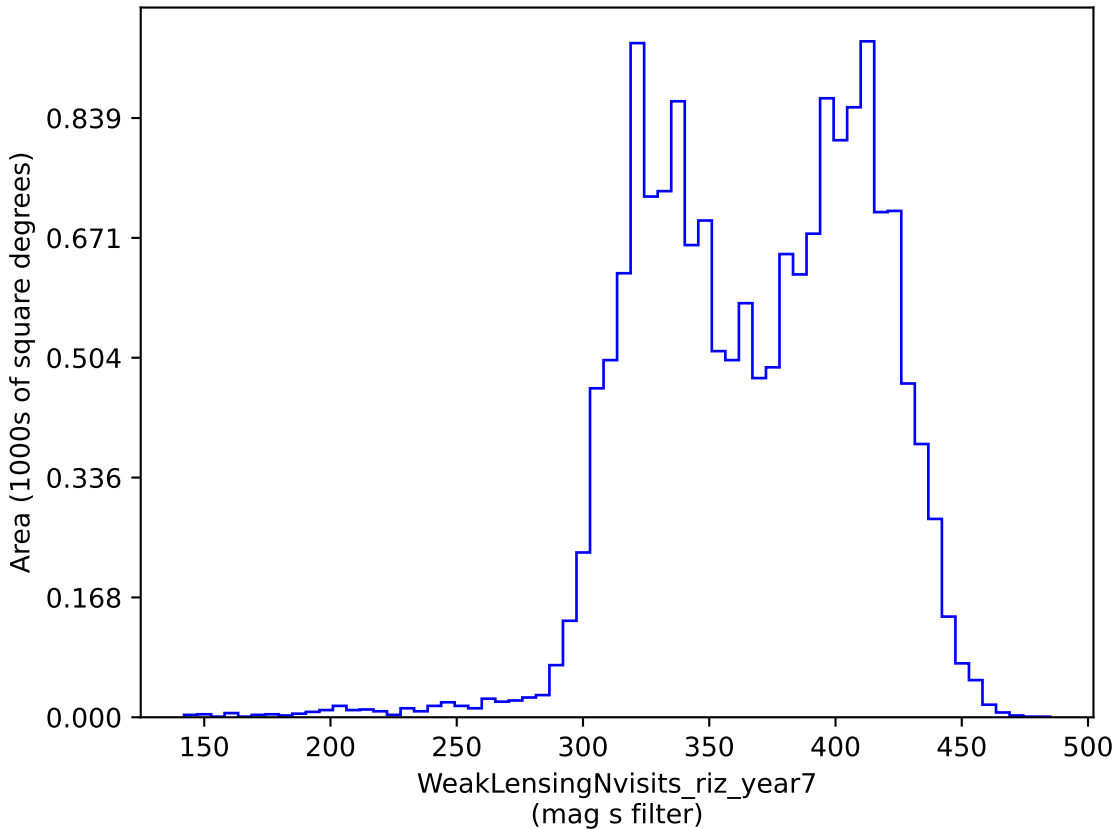
baseline_v3.3_10yrs gri band non-DD: WeakLensingNvisits_riz_year7
