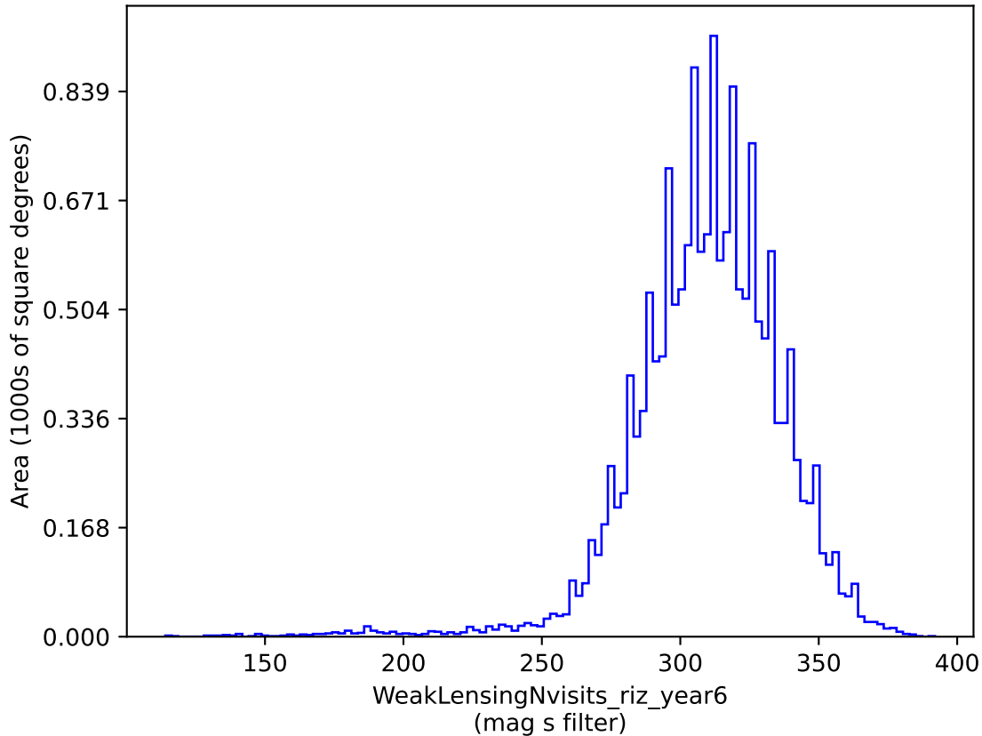
baseline_v3.3_10yrs gri band non-DD: WeakLensingNvisits_riz_year6
