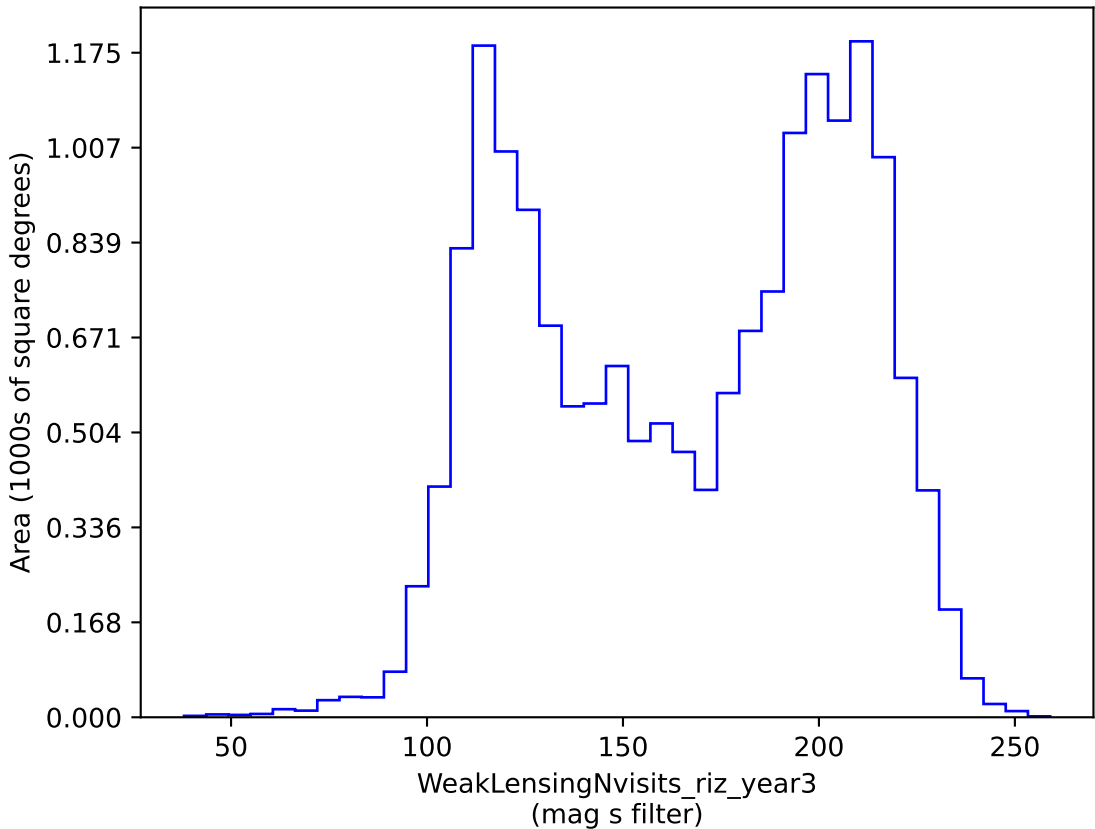
baseline_v3.3_10yrs gri band non-DD: WeakLensingNvisits_riz_year3
