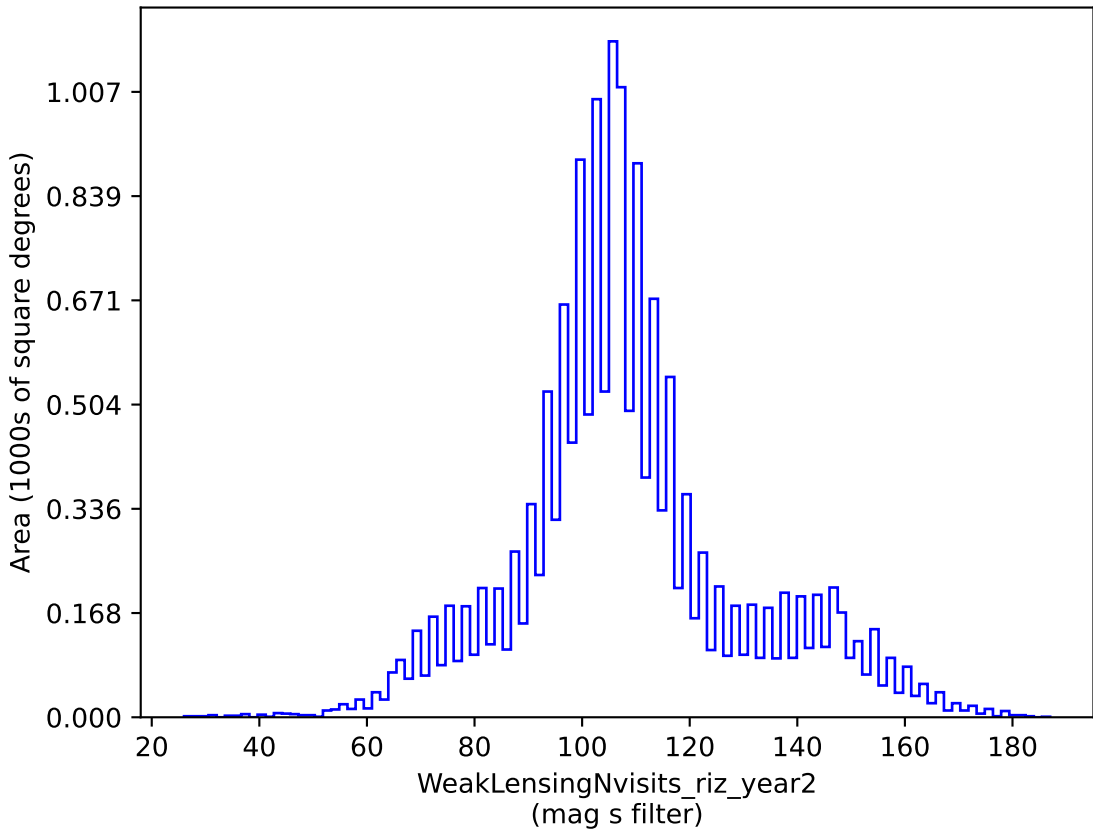
baseline_v3.3_10yrs gri band non-DD: WeakLensingNvisits_riz_year2
