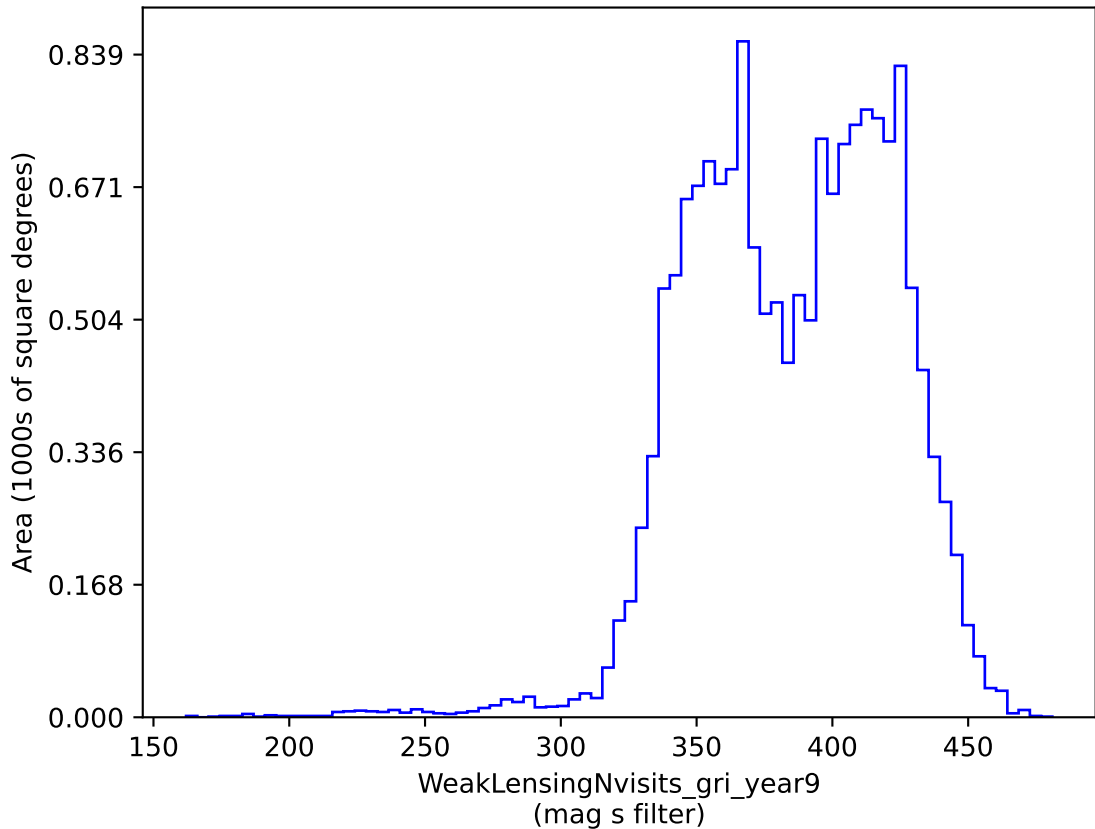
baseline_v3.3_10yrs gri band non-DD: WeakLensingNvisits_gri_year9
