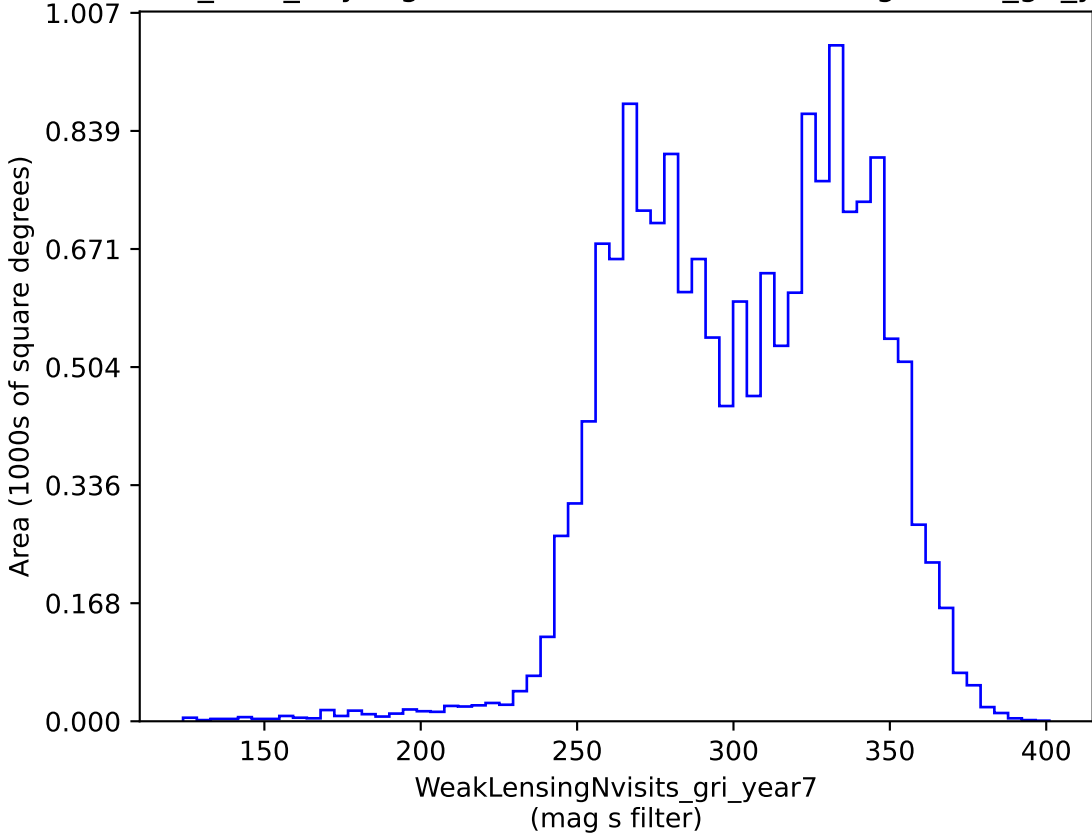
baseline_v3.3_10yrs gri band non-DD: WeakLensingNvisits_gri_year7
