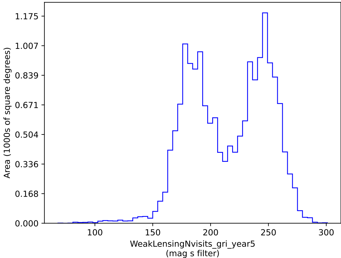
baseline_v3.3_10yrs gri band non-DD: WeakLensingNvisits_gri_year5
