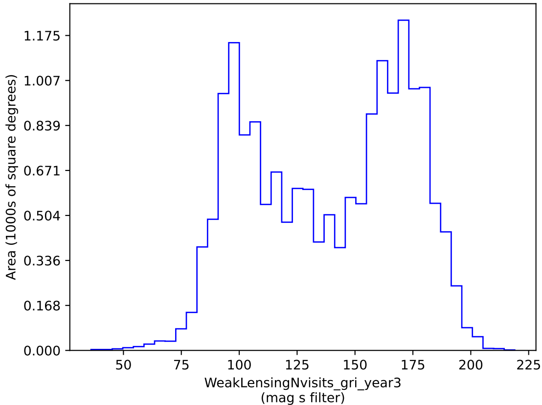
baseline_v3.3_10yrs gri band non-DD: WeakLensingNvisits_gri_year3
