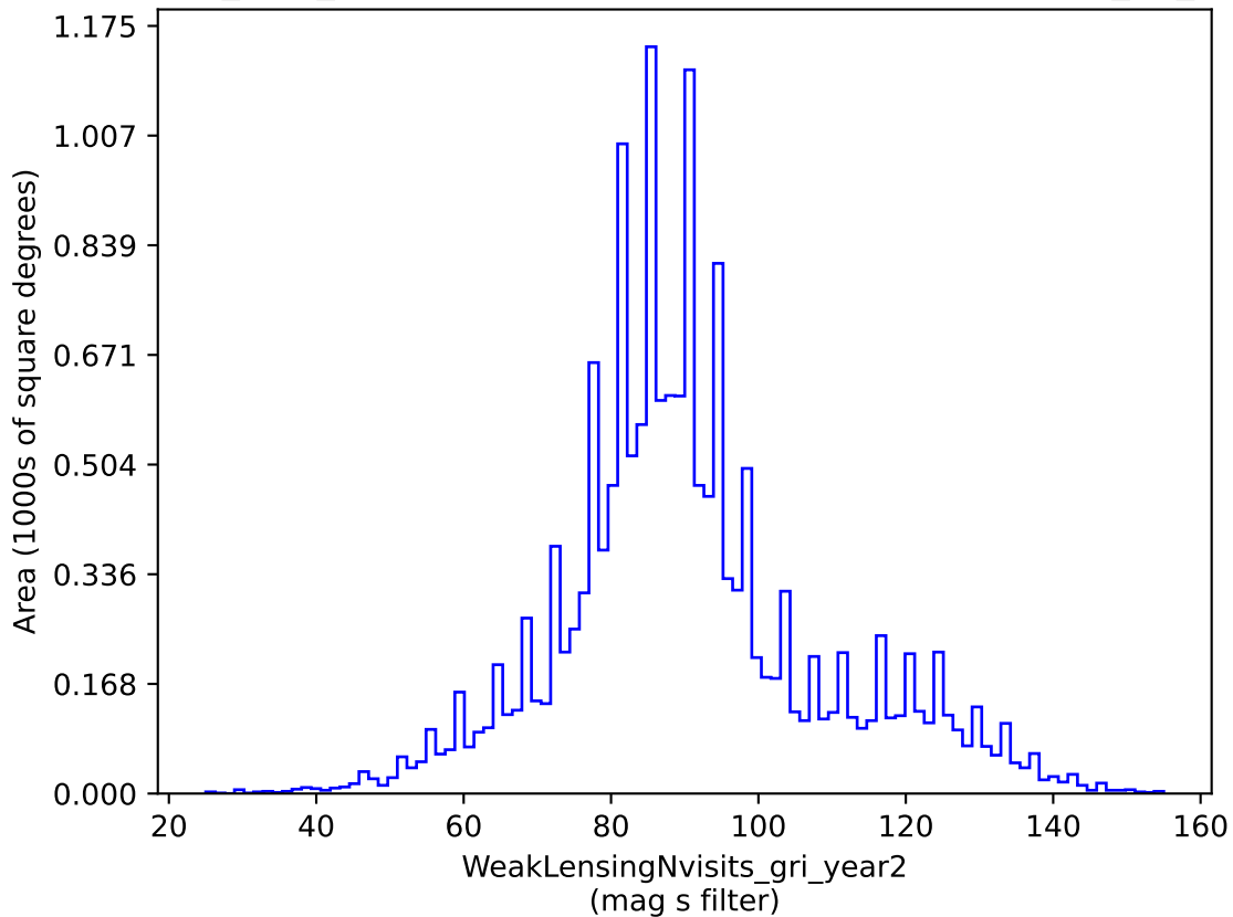
baseline_v3.3_10yrs gri band non-DD: WeakLensingNvisits_gri_year2
