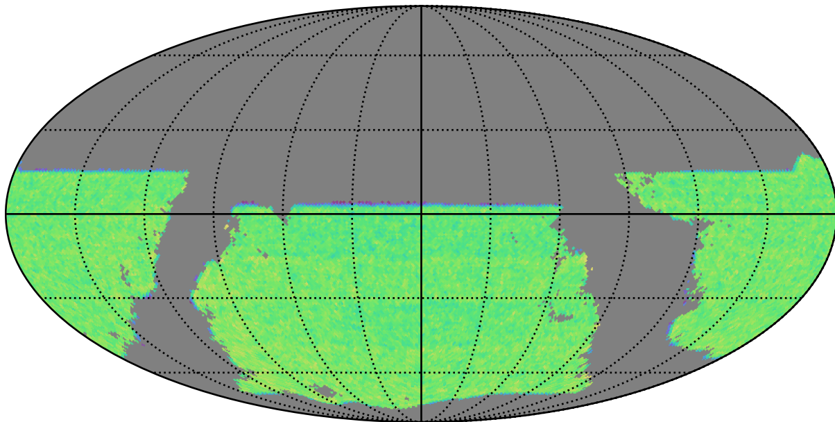
baseline_v3.3_10yrs gri band non-DD: WeakLensingNvisits
