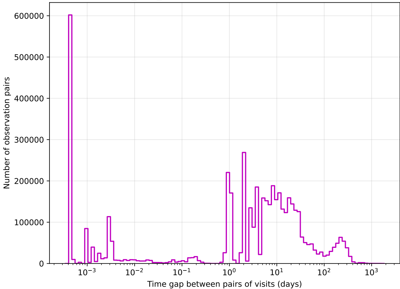
baseline_v3.3_10yrs z band: Tgaps observationStartMJD
