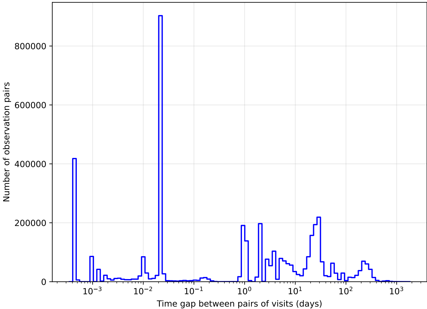
baseline_v3.3_10yrs y band: Tgaps observationStartMJD
