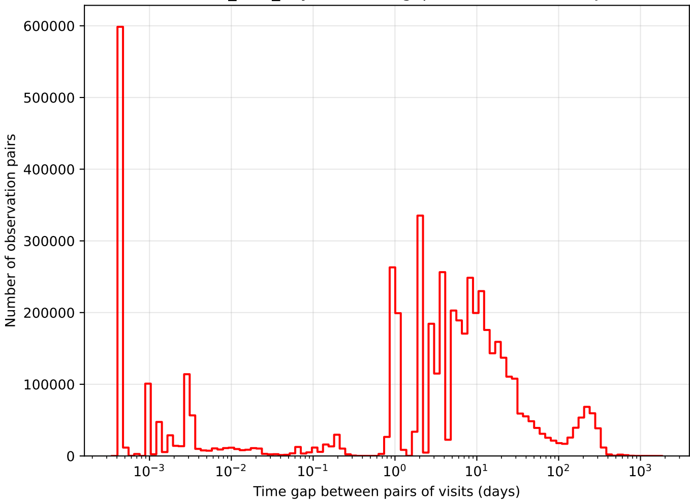
baseline_v3.3_10yrs i band: Tgaps observationStartMJD
